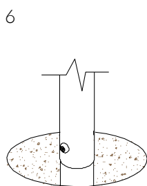
6 Compact base of hole with 50mm of aggregate. Lower ground Fix post attached to instrument into hole (check instrument straight and level before filling with concrete)
