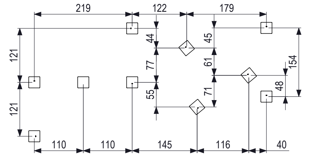
Foundation plan SCALE 1:50
